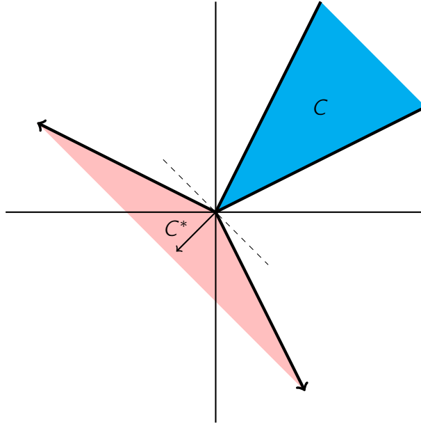
Figure 4: A cone and its polar cone.
