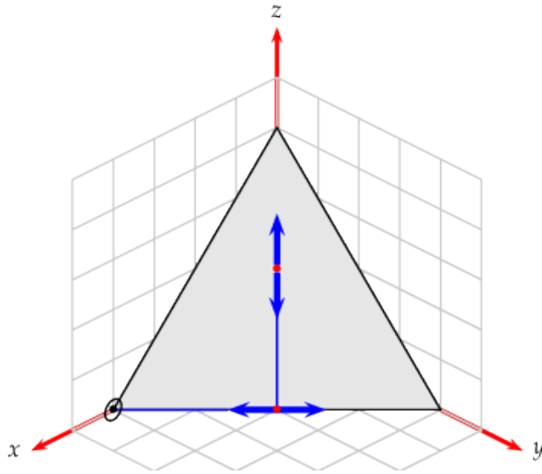
Figure 3: Finding a vertex.
